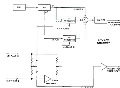
Figure 6. C-QUAM transmitter block diagram.
