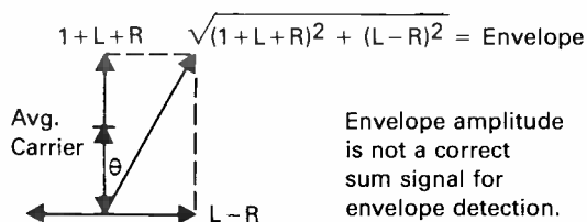
Figure 1. Basic quadrature AM (QUAM).
